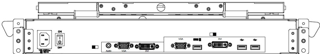
Rear view of ATZ LKD19D2V
