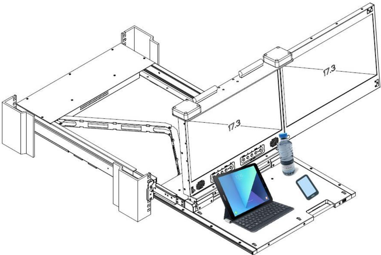
Dual-Rail design w/Retractable Tray
