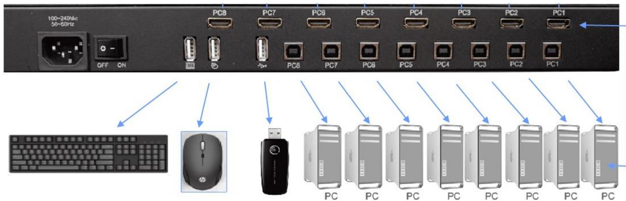
Figure 3. Computer/Server Installation
