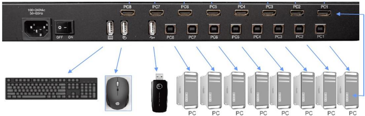
Figure 3. Computer/Server Installation
